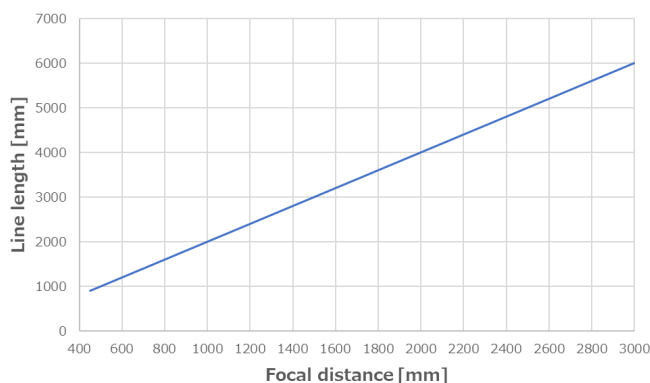
Focal distance vs Line length (FA:90°)
