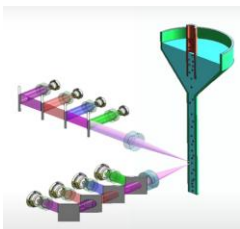
Flow cytometry
